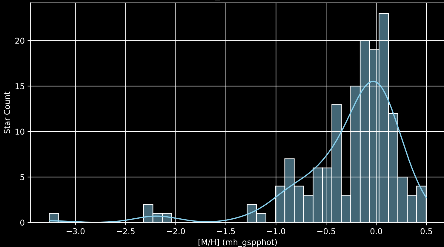
APOGEE DR17 Field: [083+04 [M/H] (mh_gspphot) (n= 155)
