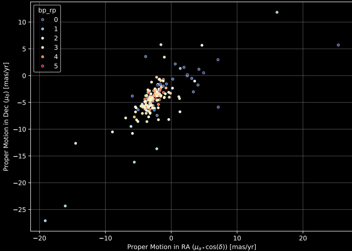
APOGEE DR17 Field: [083+04] Proper Motion Diagram (n= 161)
