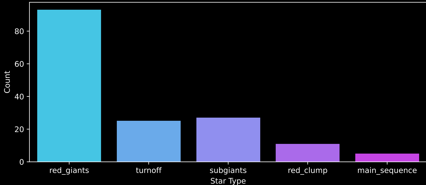
APOGEE DR17 Field: [083+04] Count plot of Star Type
