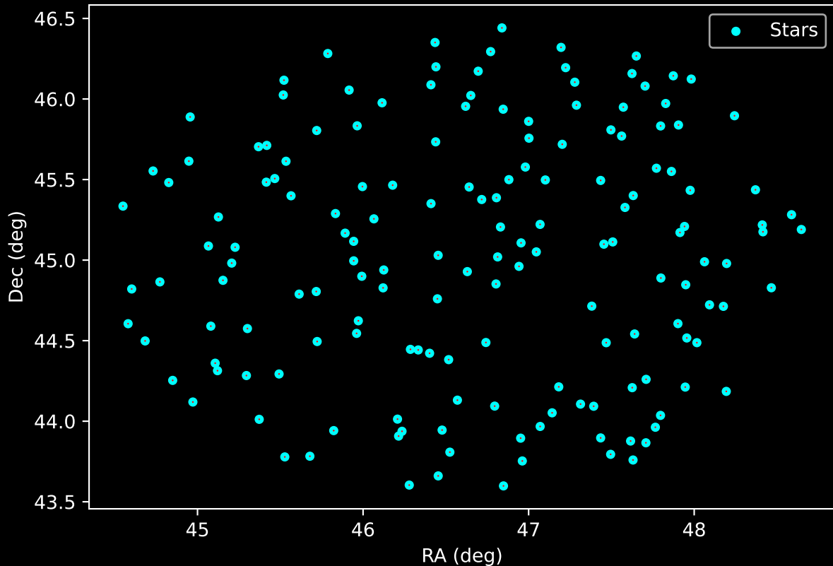
APOGEE DR17 Field: [083+04] Proper Motion Vectors for Gaia Star Field (n= 161)
