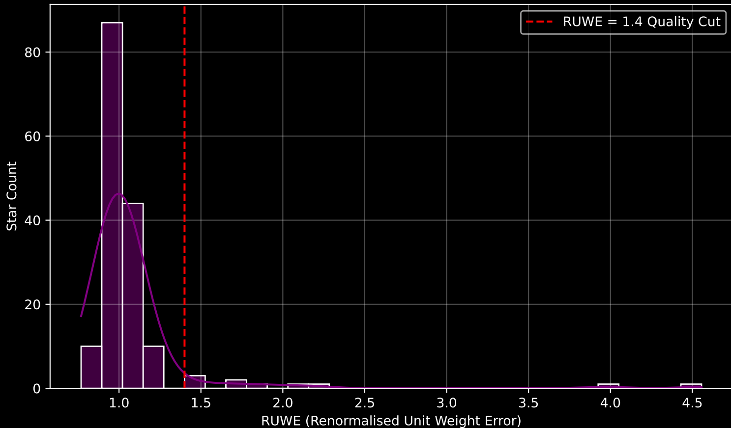
GAPOGEE DR17 Field [083+04] RUWE Distribution (n= 161)
