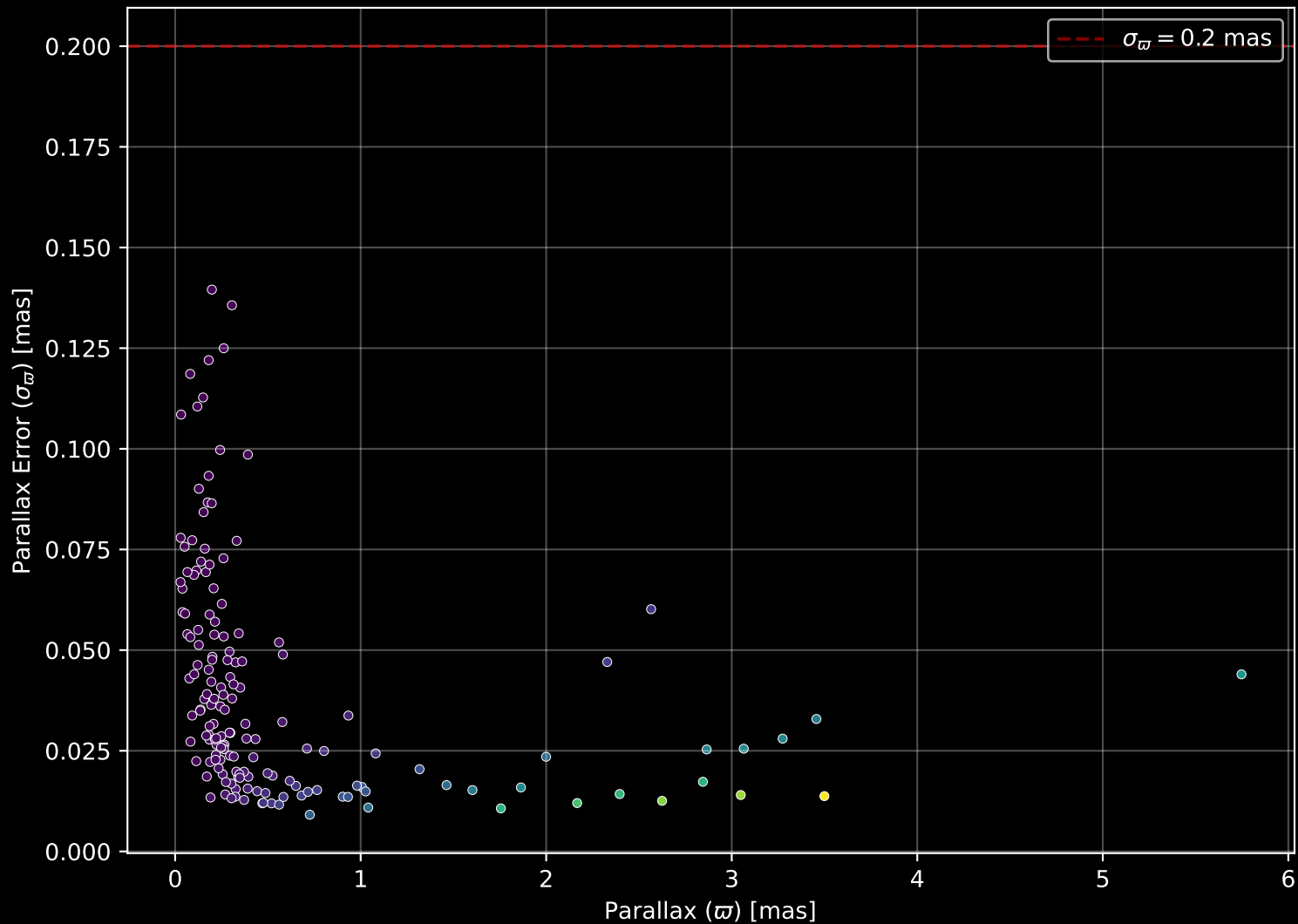
APOGEE DR17 Field: [083+04] Parallax Quality (n= 161)
